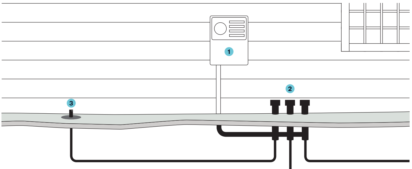
Automatic sprinkler system Diagram
