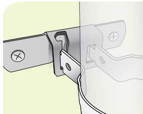
Step 2 Install pipe as required - can be pre-hung
