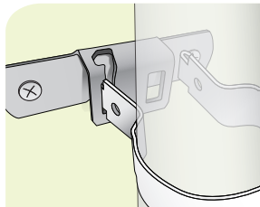
Step 2 Install pipe as required - can be pre-hung
