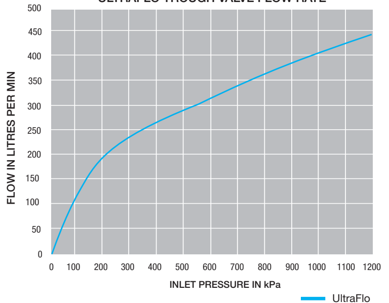
ULTRAFLO TROUGH VALVE FLOW RATE
