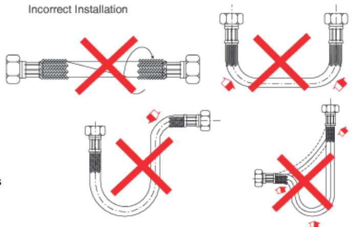
Incorrect Installation
